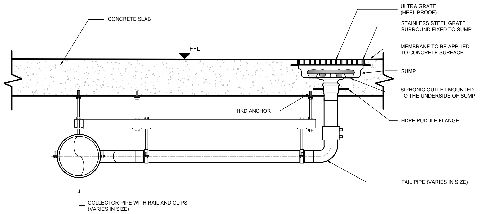
TYPICAL SLAB BRACKETING SECTION SCALE: NTS INDICATIVE ONLY
