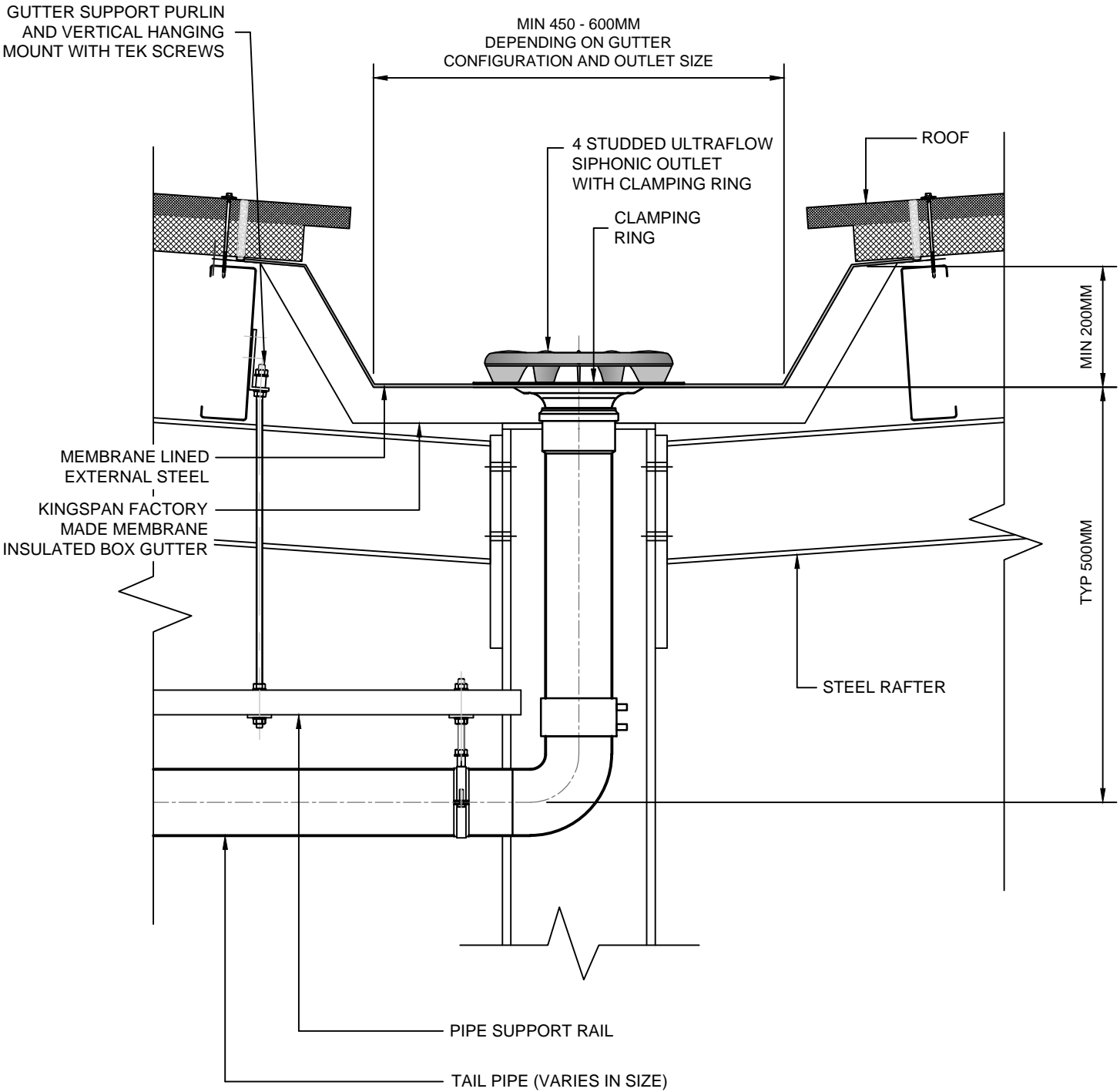
TYPICAL KINGSPAN VALLEY GUTTER DETAIL WITH SIPHONIC OUTLET SCALE: NTS INDICATIVE ONLY
