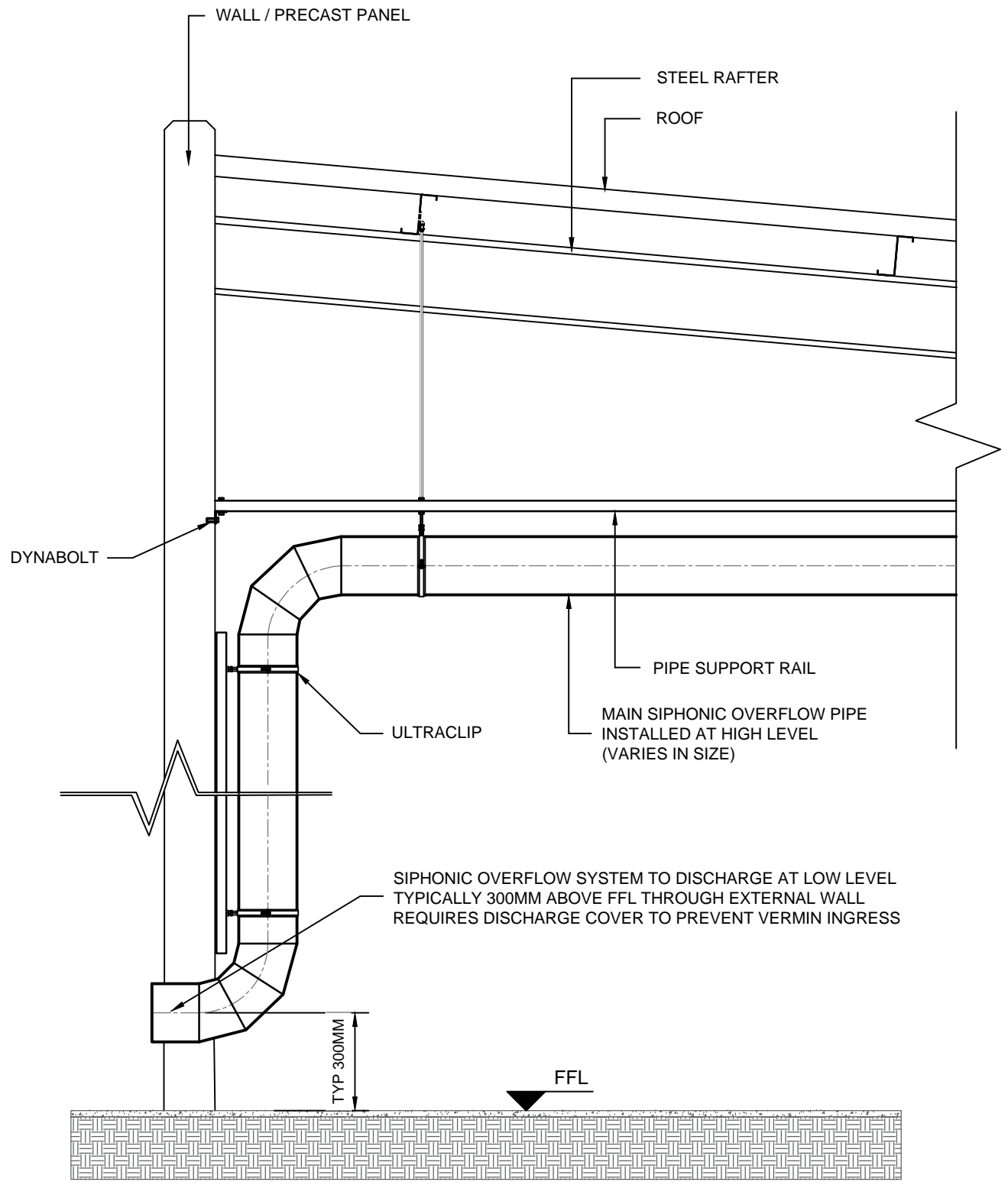
TYPICAL SIPHONIC OVERFLOW - LOW LEVEL DISCHARGE SCALE: NTS INDICATIVE ONLY
